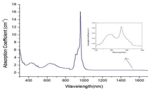
Cr14 Absorption
