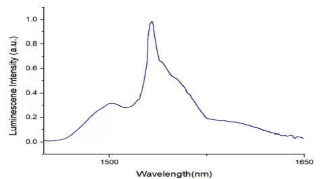
Cr14 Emission
