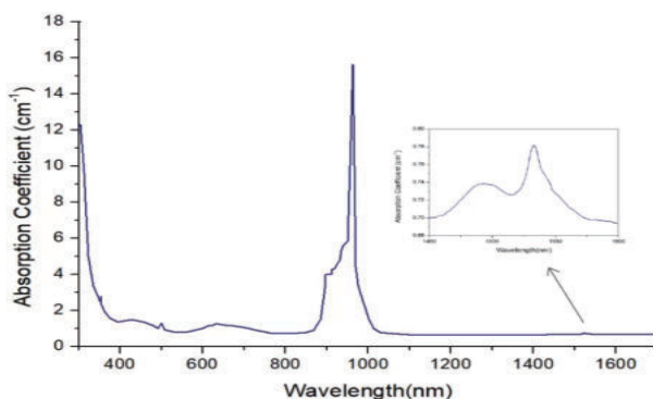
CrE5 Absorption
