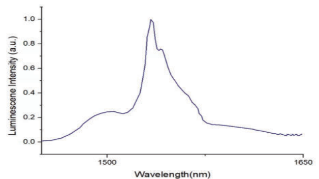
CrE5 Emission
